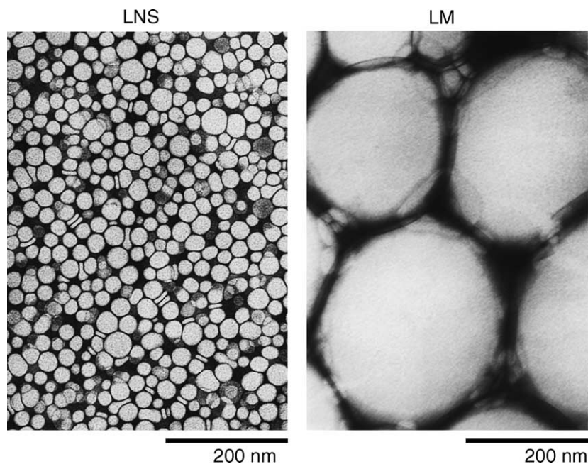
Fig. 2. Electron micrographs of negatively stained LNS and LM.
