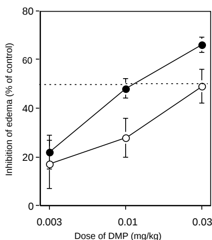
Fig. 8. Dose–response curves of lipid emulsions in the inhibition of carrageenin-induced paw edema in rats. Pharmacological potentials of lipid emulsions evaluated as inhibiting carrageenin-induced paw edema in rats. Each point represents the mean \pm S.D. of six rats. Closed circles, LNS; open circles, LM.
