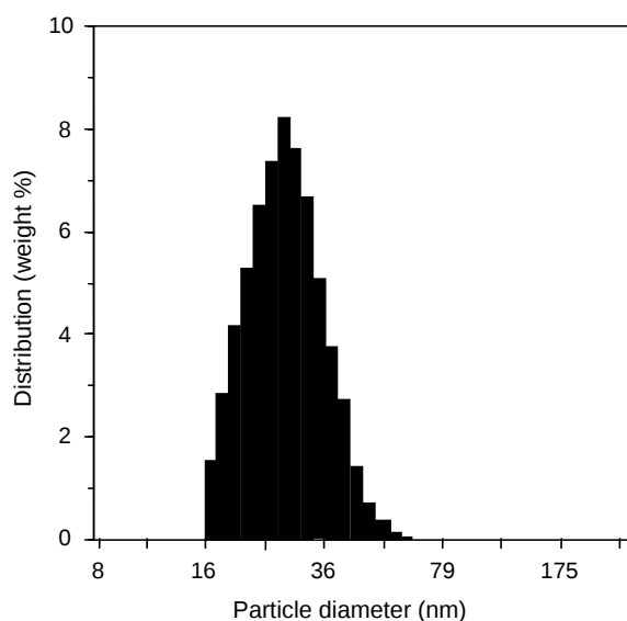
Fig. 1. Distribution of LNS particle diameters measured by dynamic laser light-scattering spectrophotometry.
